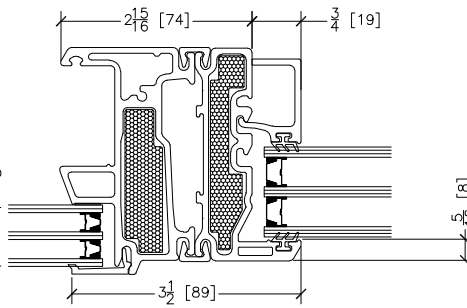
⑨ MULLION: 800 SLIDER / 328 FIXED
