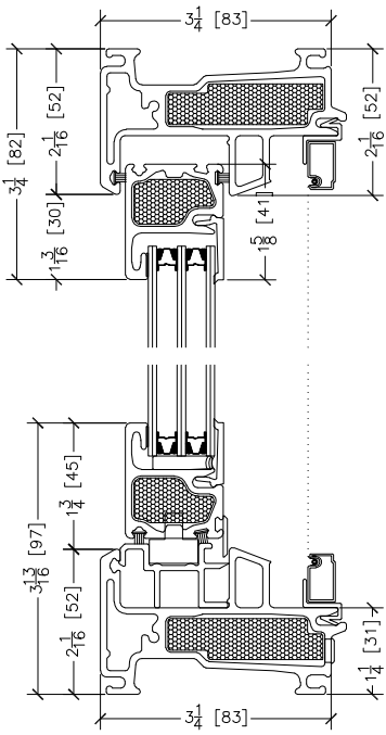
② 800 SLIDER SILL
